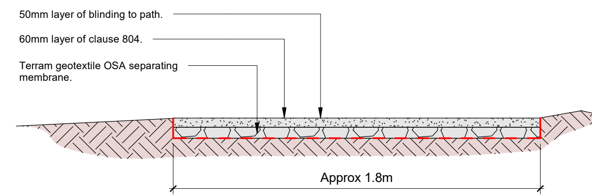
2 Proposed New Path 1 : 20
