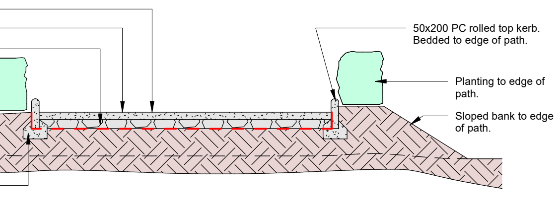
7 Proposed New Ramp Section 1 : 25
