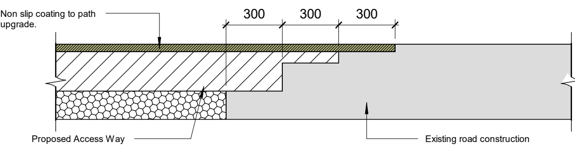
4 New Access Way Tie in Detail 1 : 20
