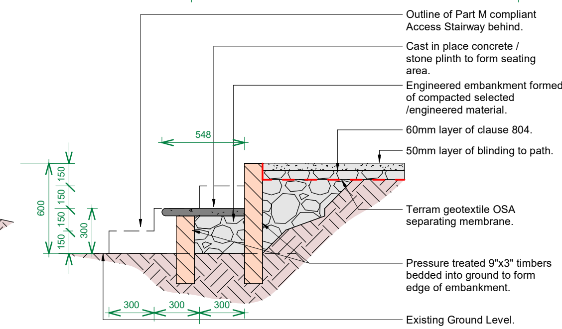
3 Abutment Seating Step 1 : 25
