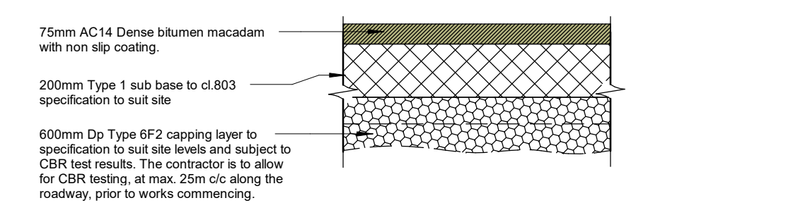
5 New Access Way Build Up 1 : 20
