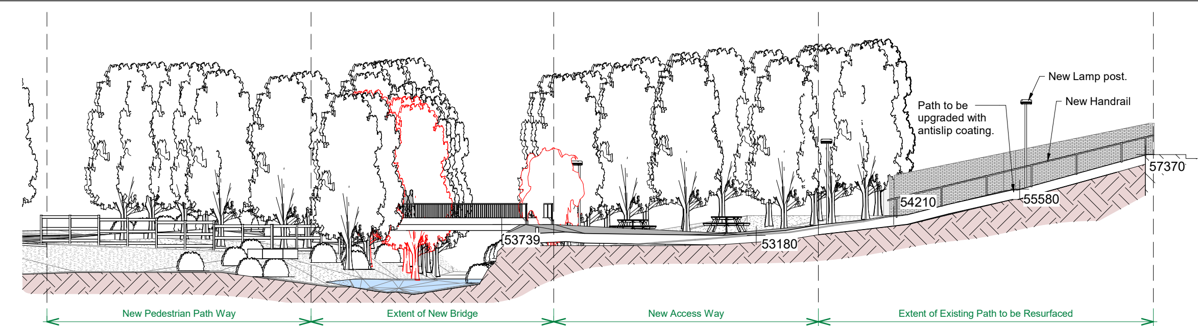
1 Long Section of Path 1 : 200
