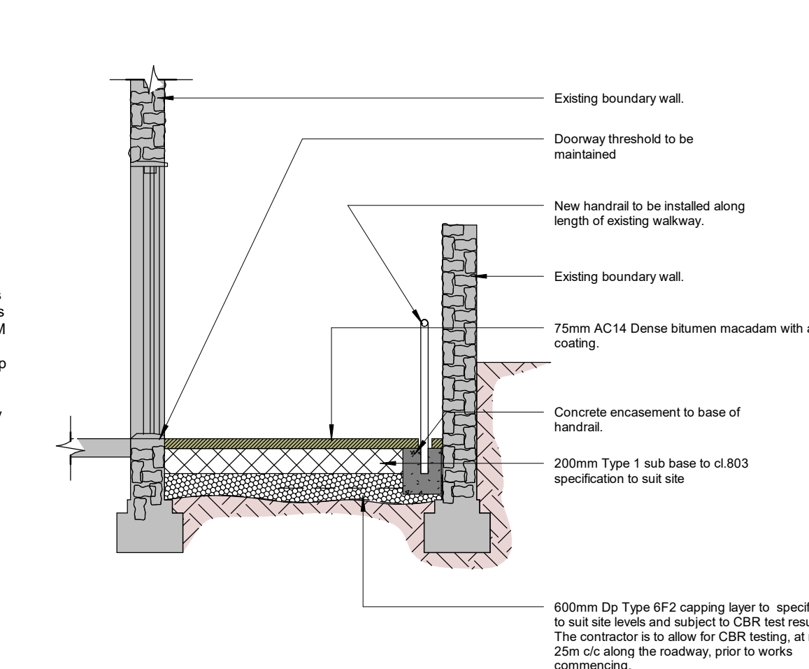
10 Existing Path Upgrade 1 : 40
